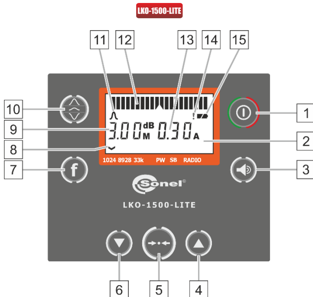
Fig. 9. Panel del receptor LKO-1500-LITE
